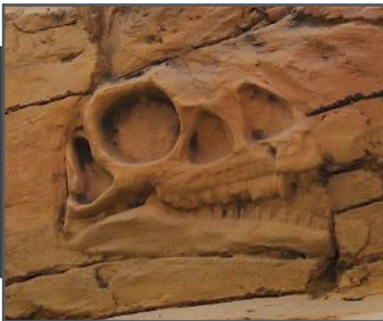
Embedded Fossils
