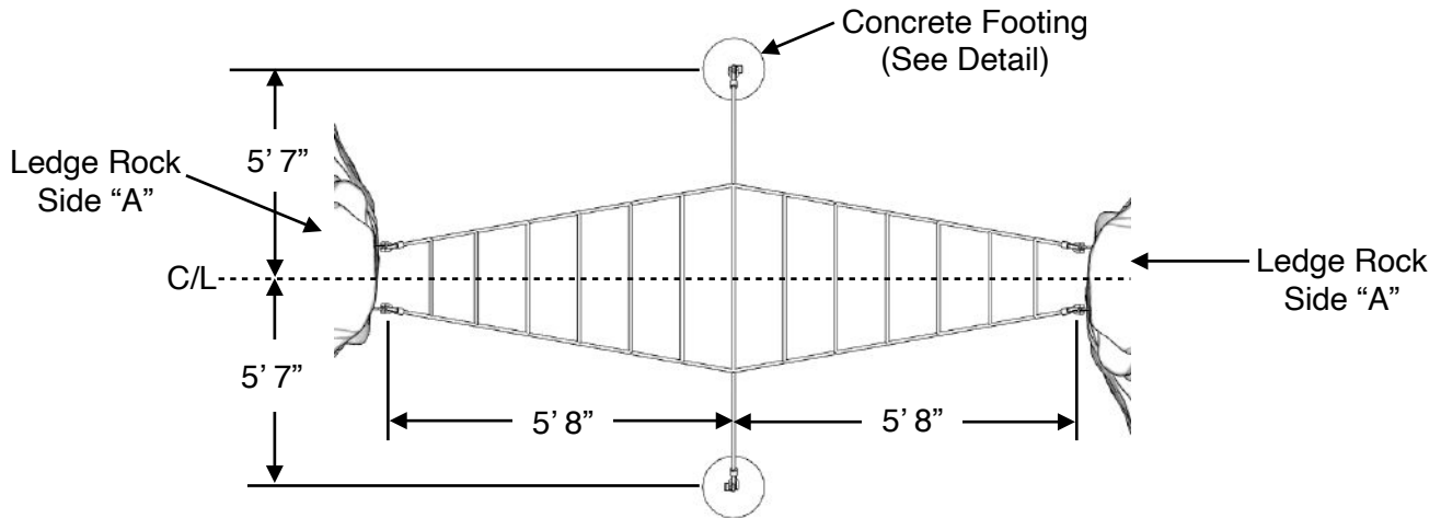
8000211 Double Ladder Net Climber Link-6 to 6
