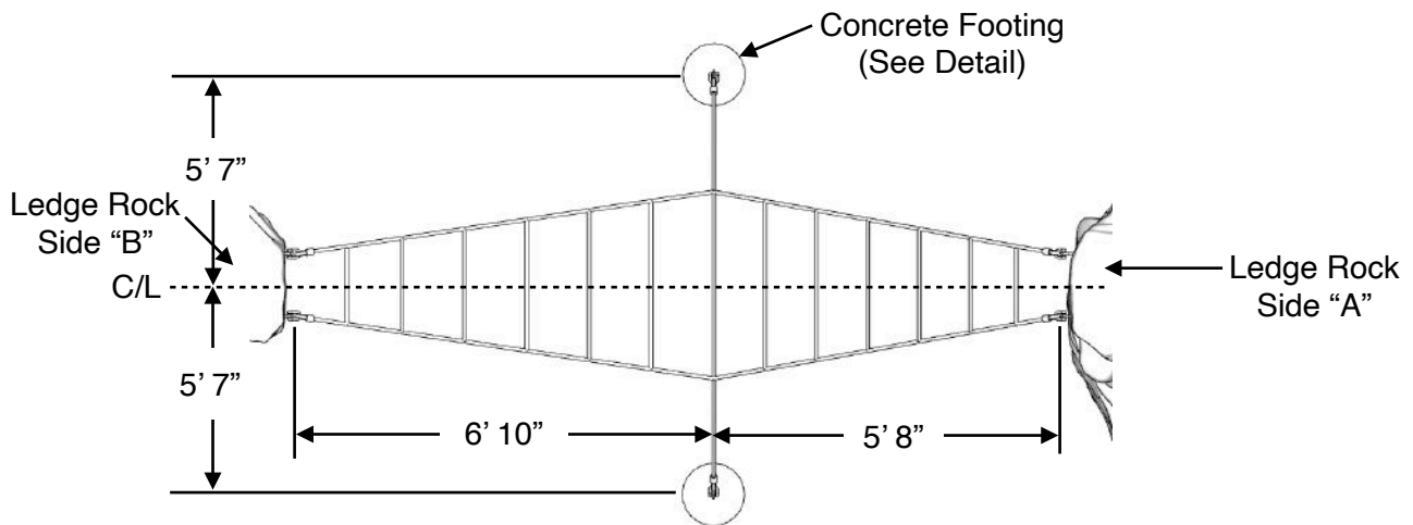
8000211 Double Ladder Net Climber Link-4 to 6
